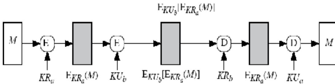
(d) Public-key encryption: confidentiality, authentication, and signature
