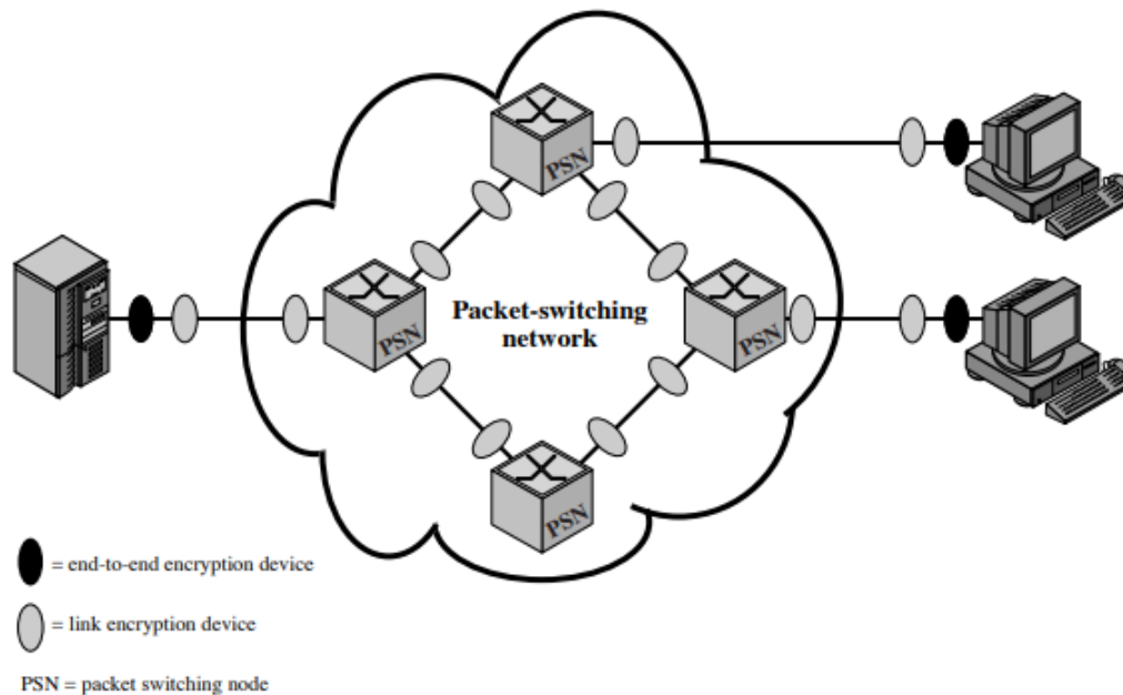
Fig 2.5.1 Encryption in Packet-Switching Networks
