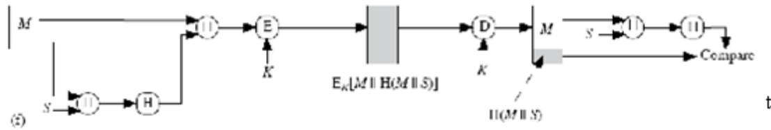
Figure 5. Basic uses of Hash function
