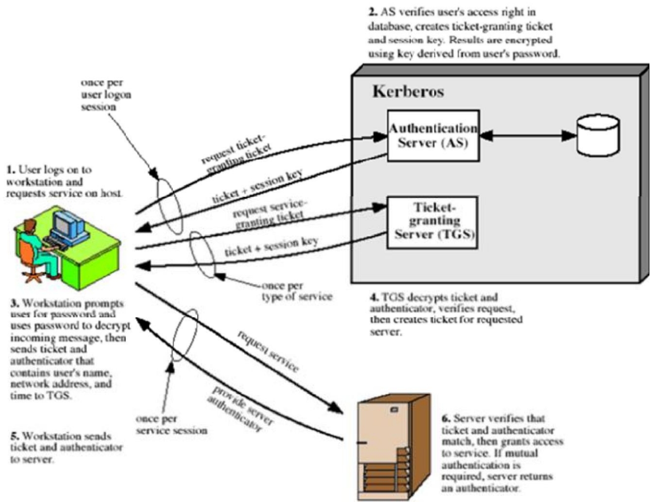
Figure 6. Kerberos 4
