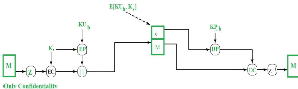
Figure 5.2 Confidentiality
